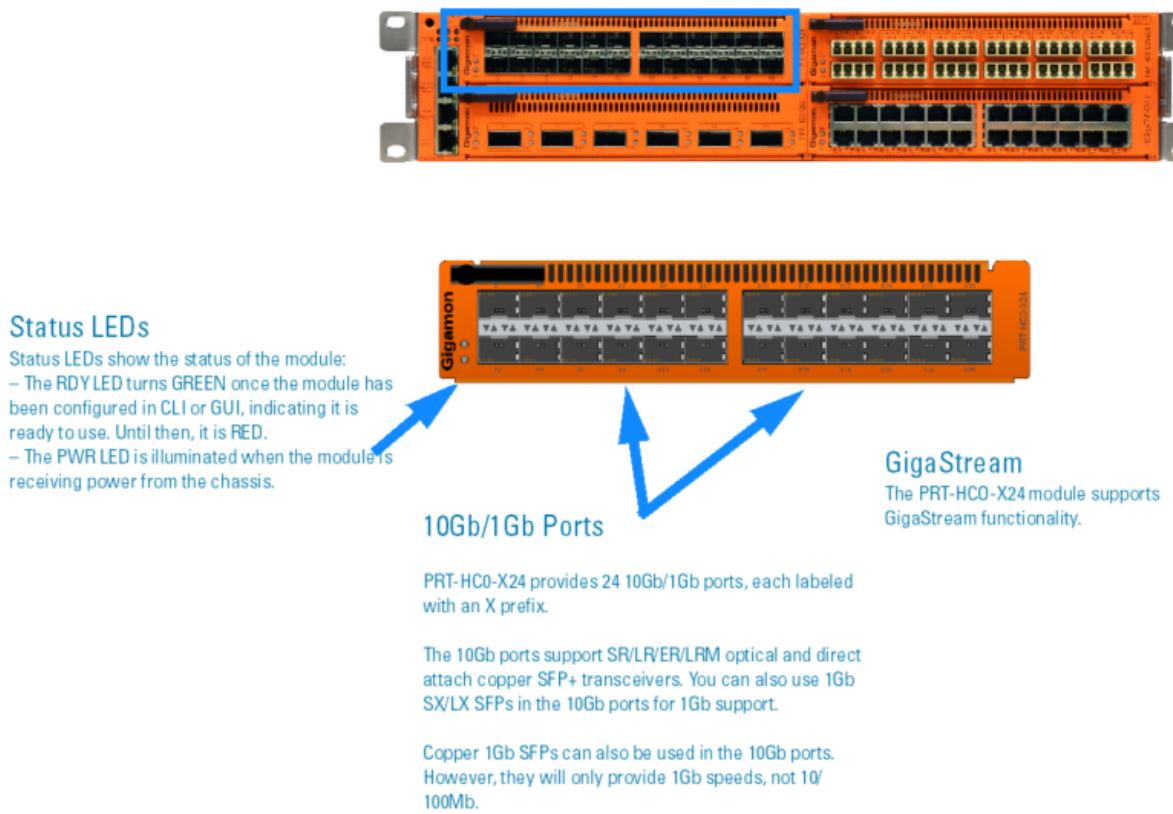
Figure 4 PRT-HC0-X24 Module
