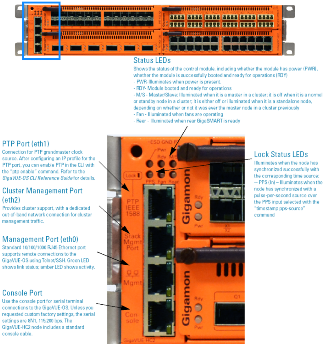
Figure 3 GigaVUE-HC2 Management Ports
